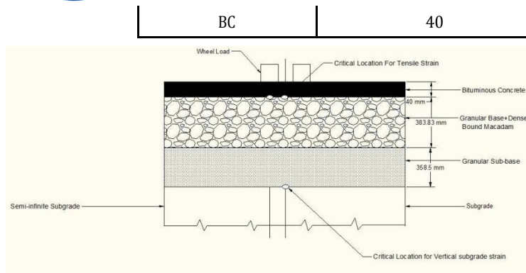
Fig.No.1 Cross-section of Flexible Pavement after Flooding.
